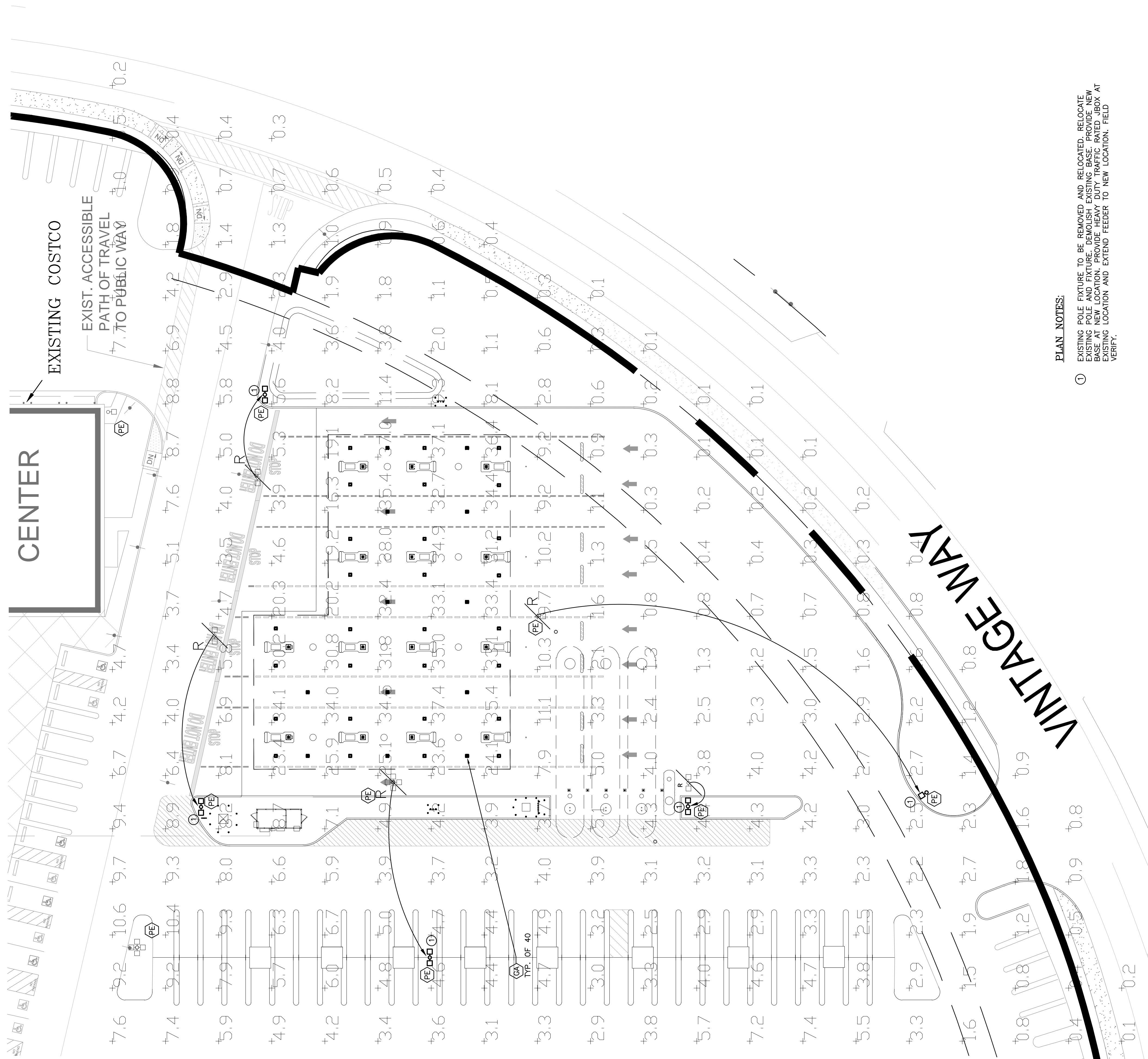
SITE PHOTOMETRIC PLAN SCALE: 1" = 20'-0"
